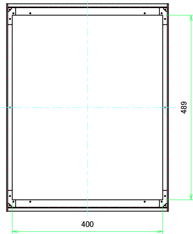
B-B (1:6)
